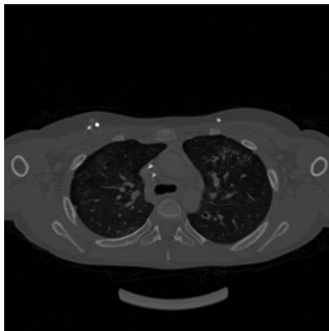
Unsegmented CT
